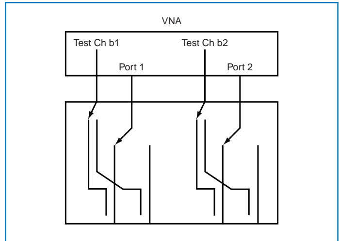
Figure 1. A coupler test set architecture is shown here: the test couplers are on the DUT-side of the multiplexing switches. As N becomes large, this test set becomes quite complex.
