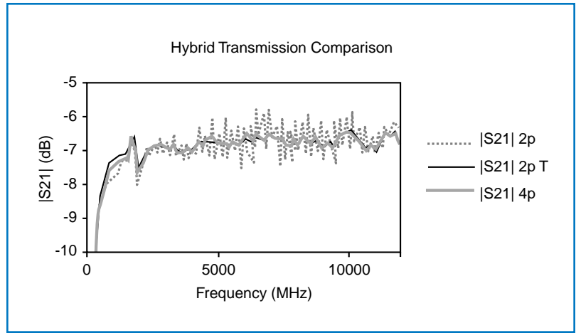
Figure 8. The measurement of transmission through a hybrid is shown here. The "4p" measurement uses the composite of covering calibrations discussed in the text. "2p T" is a 2-port measurement in which the unused ports were manually connected to metrology grade terminations. "2p" is a 2-port measurement in which the unused ports are connected to the test set but left uncorrected.
