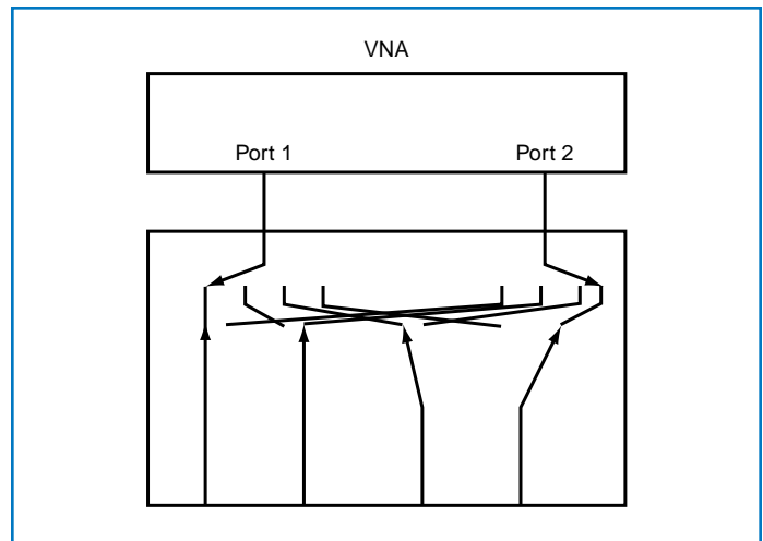
Figure 2. A no-coupler architecture for the 4x2 problem is shown here. In this case, any VNA port can be connected to any test port although this is not needed for most measurements. This test set can be simpler for large N but does have limitations.
