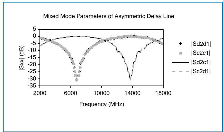
Figure 9. The microwave measurement of a very poor balanced delay line is shown here. As the length difference passes through 180 degrees, mode conversion reaches a maximum.
