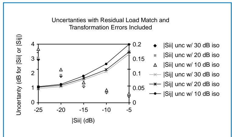
Figure 12. Uncertainties for a no-coupler test set measurement of the same path in the 8-port DUT are shown here. An added term for uncertainty in characterizing the off-state matches of the test set ports is required, but has small impact except when measuring deep match or insertion loss under poorly matched conditions.
