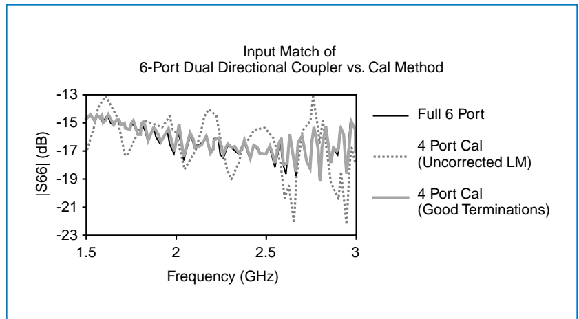
Figure 5. The input match as measured with a full 6-port cal, and two different 4-port calibrations (one where the two unmeasured ports are test-set terminated and one where they are terminated with >50 dB terminations) is shown here. The full 6 port result compares favorably to the labor intensive measurement with good terminations.
