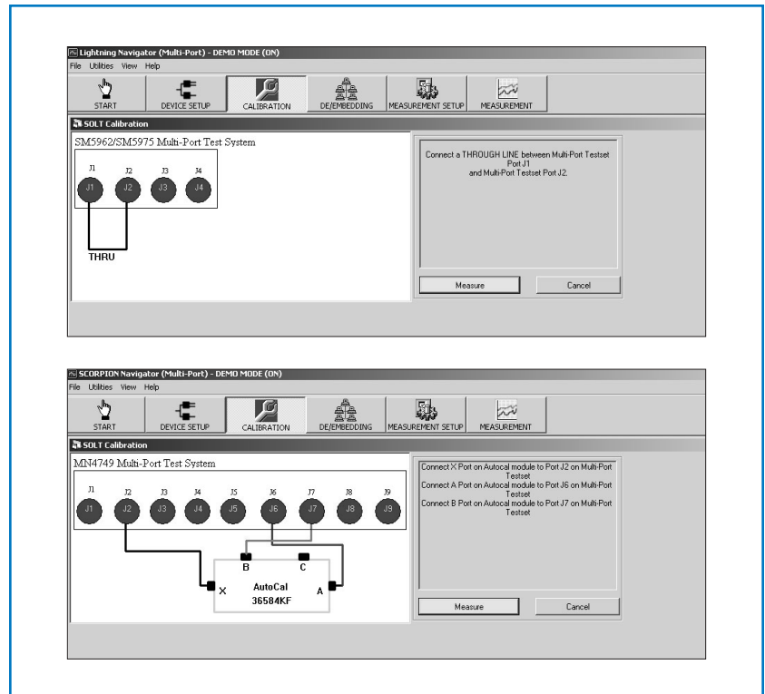
Figure 4. Example calibration screens from Navigator software are shown here for manual (top) and automatic (bottom) calibration routines. The software can assist in directing the user through the required steps and in simplifying setup tasks.
