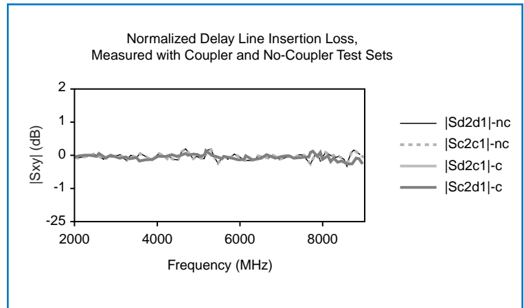
Figure 10. Normalized transmission through a delay line is shown here for measurements performed on a coupler test set and a no-coupler test set. The spread (due to line mismatch and high level noise from this very fast measurement) is about the same.
