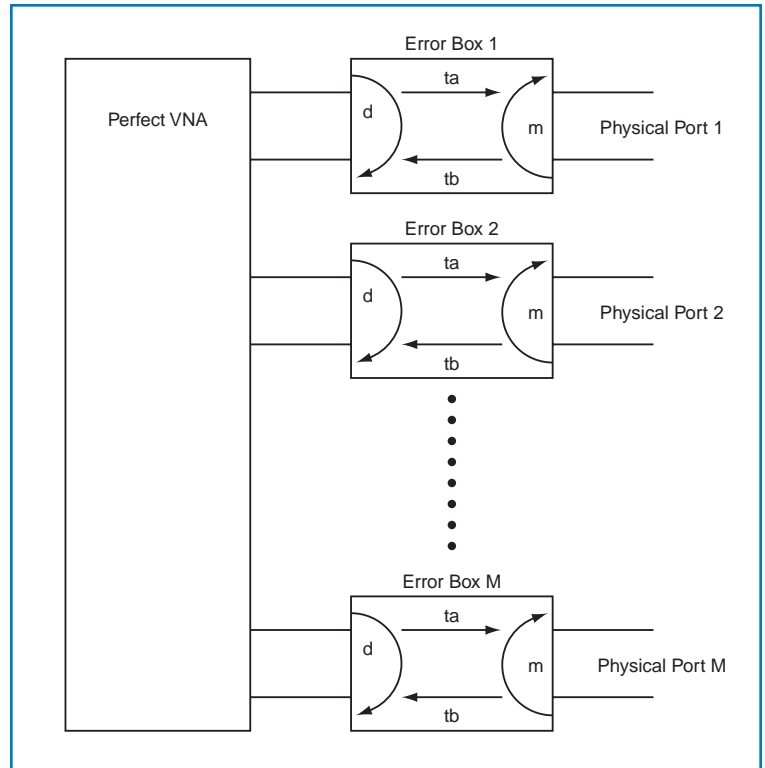
Figure 3. A diagram is shown here of the error boxes for an M port calibration. The “d” denotes a directivity term, the “m” a match term (source match or load match) and the “ta” and “tb” denote portions of the tracking terms. The product “ta*tb” within an error box is a reflection tracking term while the product of ta from one error box with tb from another error box is the transmission tracking term for that path.
