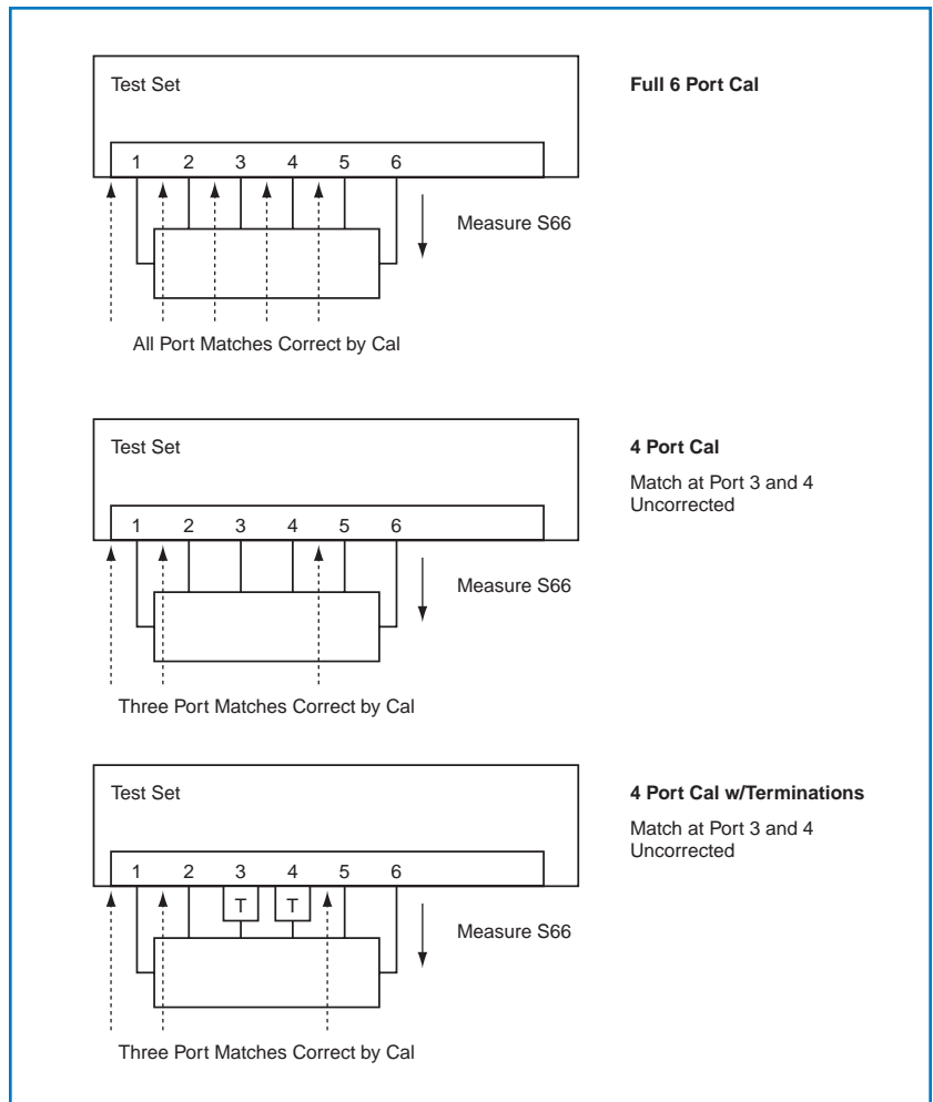
Figure 6. An illustration of the different measurements in figure 5 is shown here. At issue is how the matches presented to all of the indirect ports are handled.
