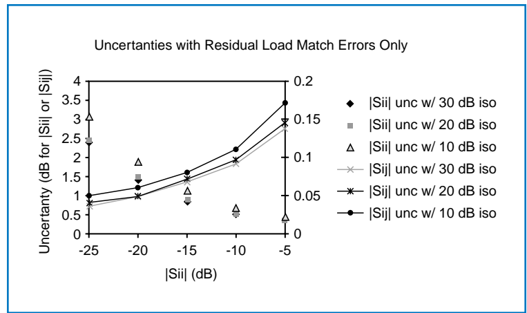
Figure 11. Uncertainties applicable to a coupler test set measuring a low-loss path on an 8 port DUT are shown here. As long as the isolation to the other ports is high, the load match impact is nil. At lower levels of isolation, an added term from load match residuals can increase uncertainty.
